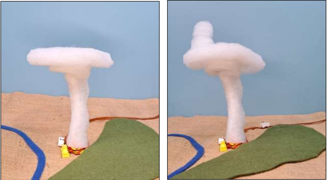
Smoke plume under inversion layer and showing the inversion layer weakening.
